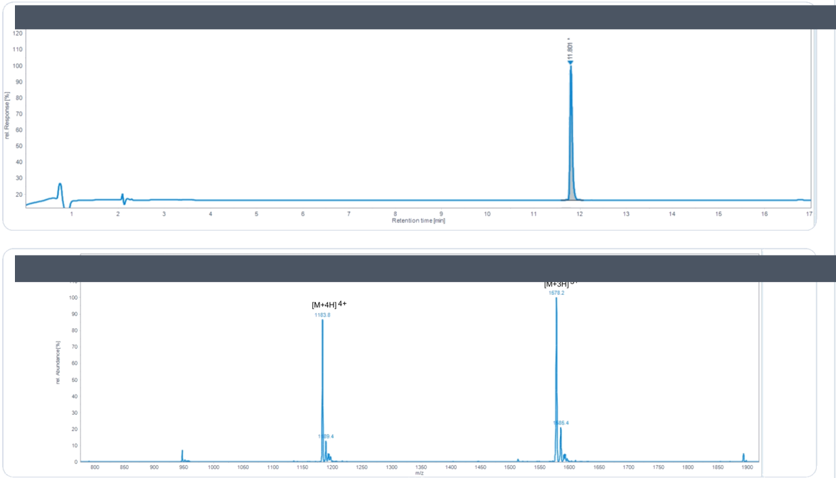
HPLC Chromatogram · Retention Time 11.801 min
