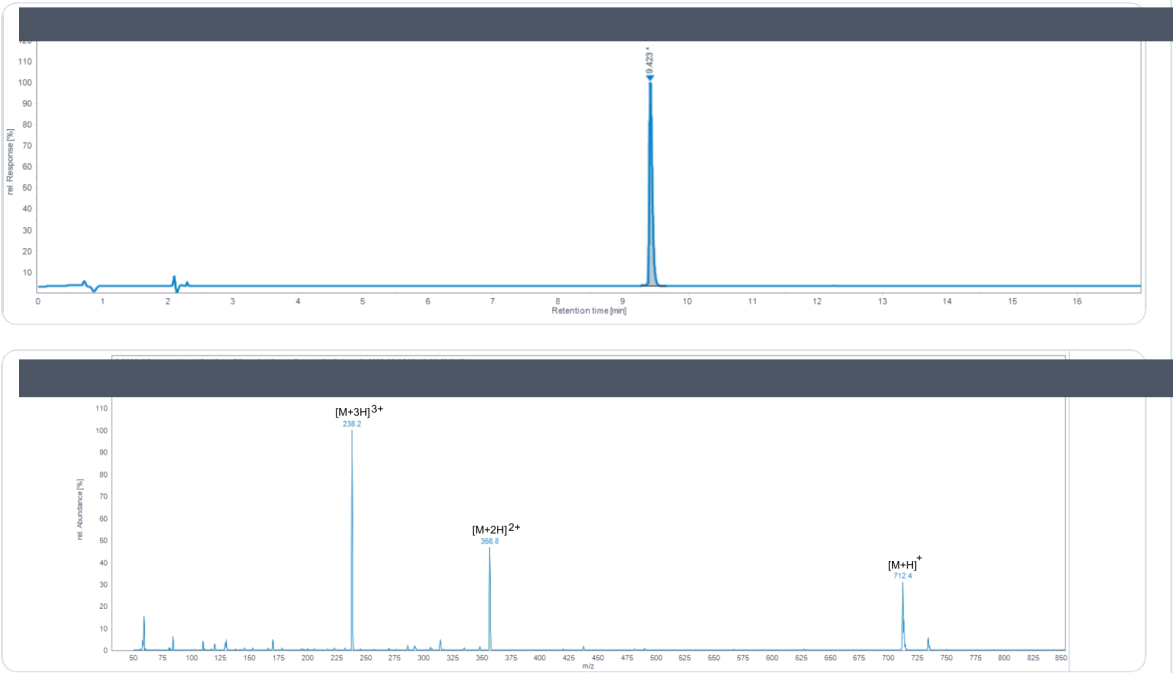
HPLC Chromatogram · Retention Time 9.423 min
